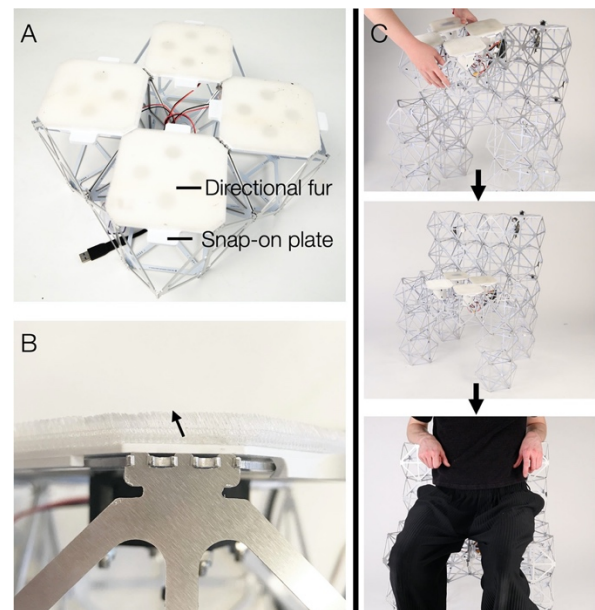
Figure 15: Overview of the Slowbot. A) Bottom view of the Slowbot, showing the directional fur modules. B) Close-up view of directional fur, with an arrow indicating its orientation. C) Installing the slowbot into the Chairemin.
