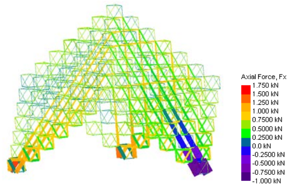
FIGURE 10: ANALYSIS RESULTS FOR WIND LOAD ON SHELTER STRUCTURE. AXIAL FORCES RESULTING FROM 80 KPH WIND LOADS
