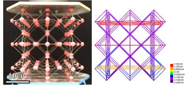
FIGURE 15: (L) 3x3x3 VOXEL TEST SPECIMEN BETWEEN TWO PLATES FOR INSTRON TESTING, (R) BEAM MODELING RESULTS FOR LOAD AT FAILURE P = 2750 N.
