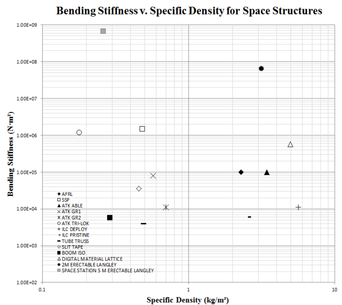
FIGURE 18: BENDING STIFFNESS V DENSITY OF SPACE STRUCTURES AND DIGITAL MATERIAL STRUCTURES. DATA FOR SPACE STRUCTURES OBTAINED FROM [24][25]
